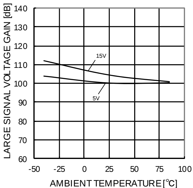
Figure 46. Large Signal Voltage Gain - Ambient Temperature ( R_L=2k\Omega )
