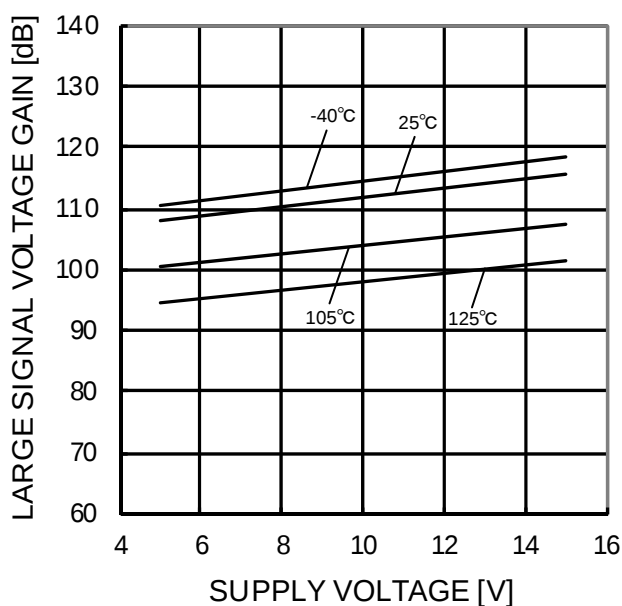
Figure 93. Large Signal Voltage Gain - Supply Voltage (RL=2kΩ)
