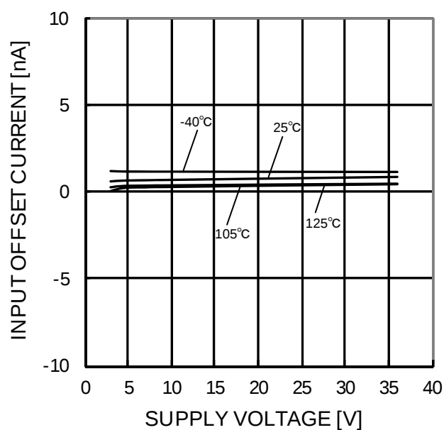
Figure 91. Input Offset Current - Supply Voltage (VICM=0V, OUT=1.4V)
