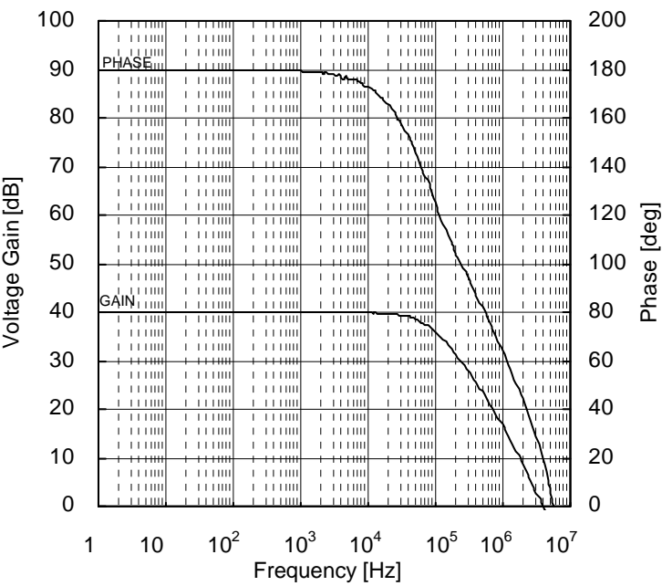
Figure 23. Voltage Gain • Phase vs Frequency (VCC/VEE=+15V/-15V, A V =40dB, R L =2kΩ, T A =25°C)
