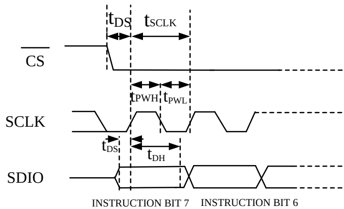
Figure 7-3. Timing Diagram for Serial Port Register Write
