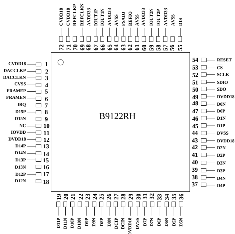
Figure 6-1 Pin Descriptions
