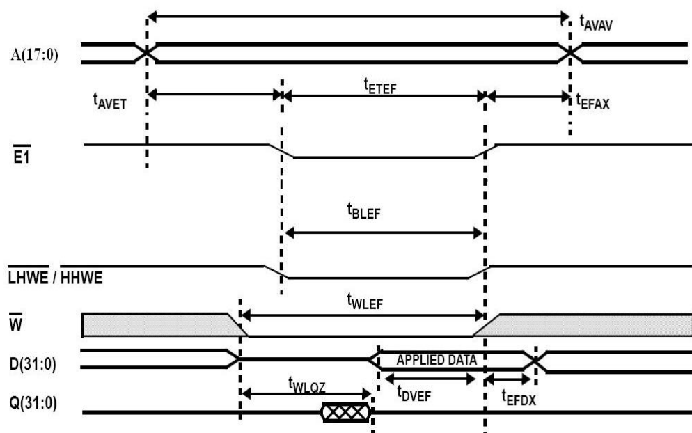
Figure 7. SRAM Write Cycle 1: \overline{W} -controlled Access
