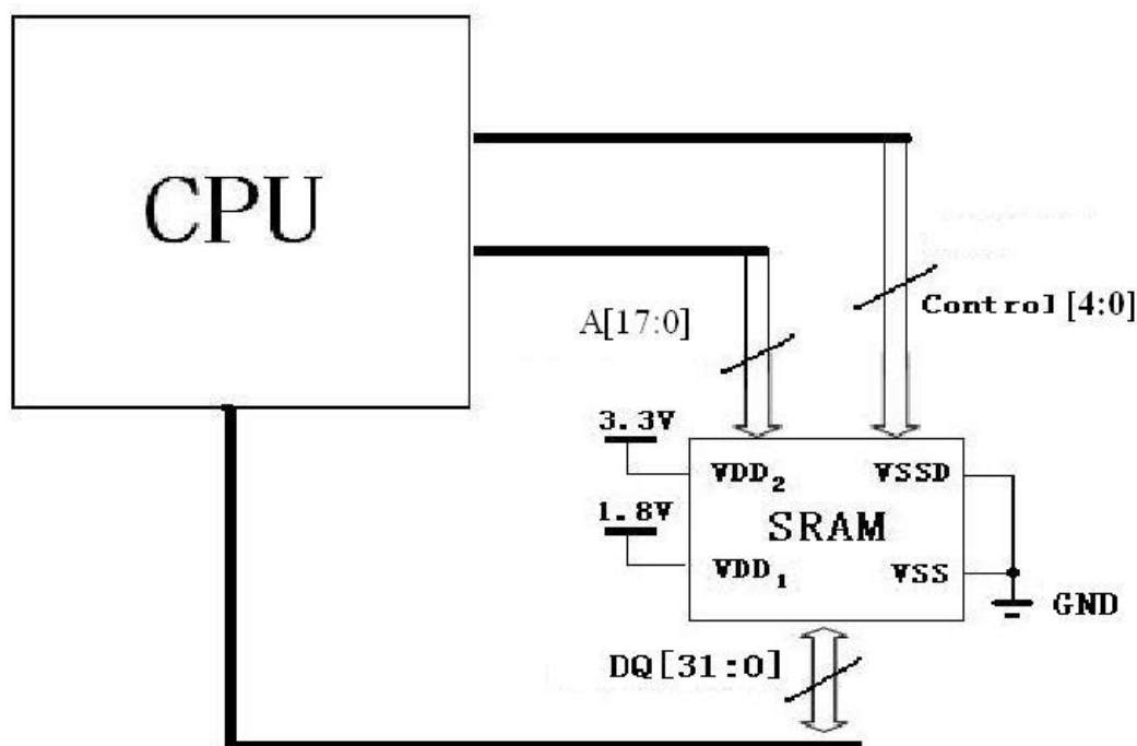
Figure 10. Typical Application
