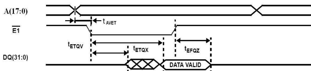
Figure 4. SRAM Read Cycle 1: Address Access
