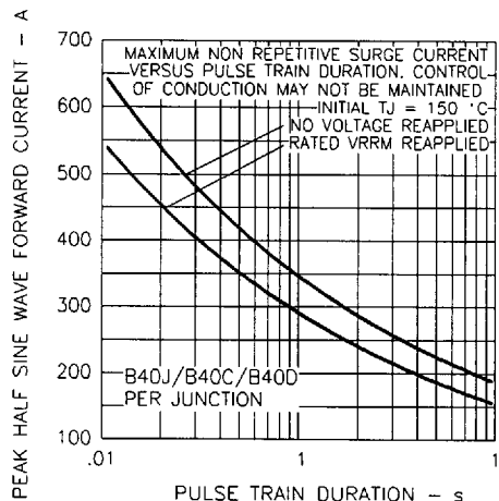
Fig. 8 - Maximum Non-Replicative Surge Current
