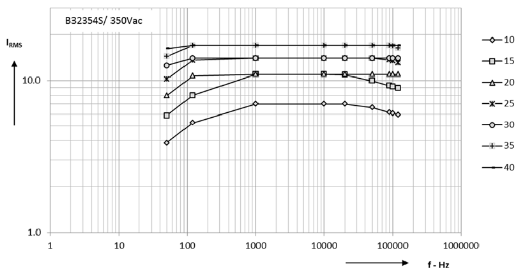
Permissible Current ( I_{rms} ) Vs Frequency at 70^{\circ}\text{C} case temperature
