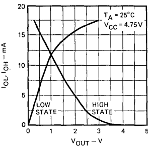
Typical Output Current Versus Voltage
