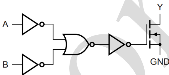
Figure 3. Logic diagram
