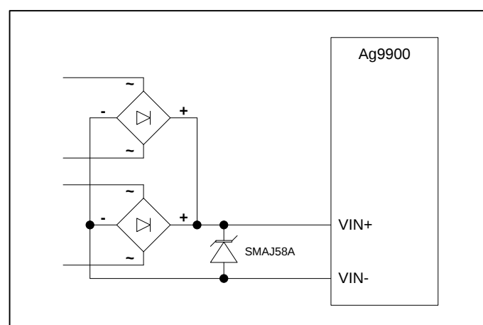
Figure 18: Ag9900 Input Protection
