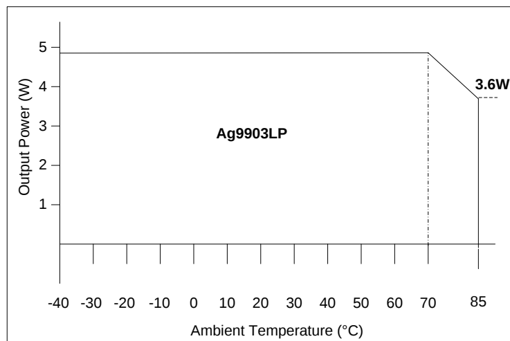
Figure 14: Ag9903LP Operating Profile
