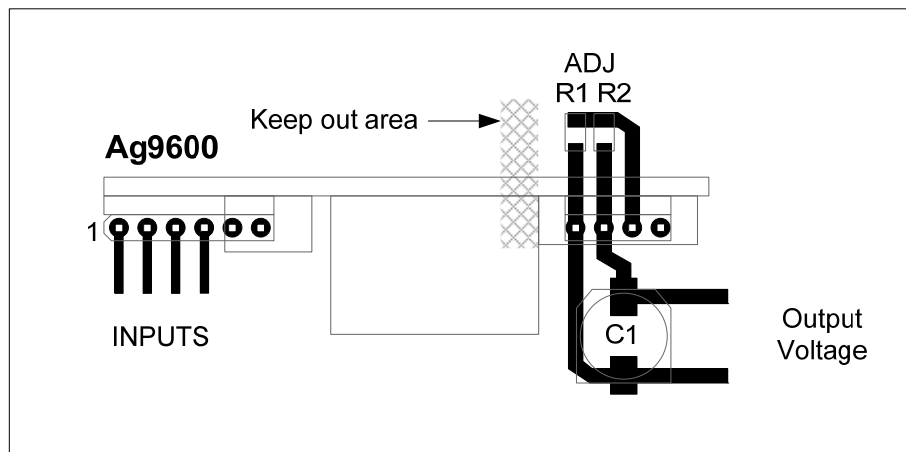
Figure 8: Typical Layout
