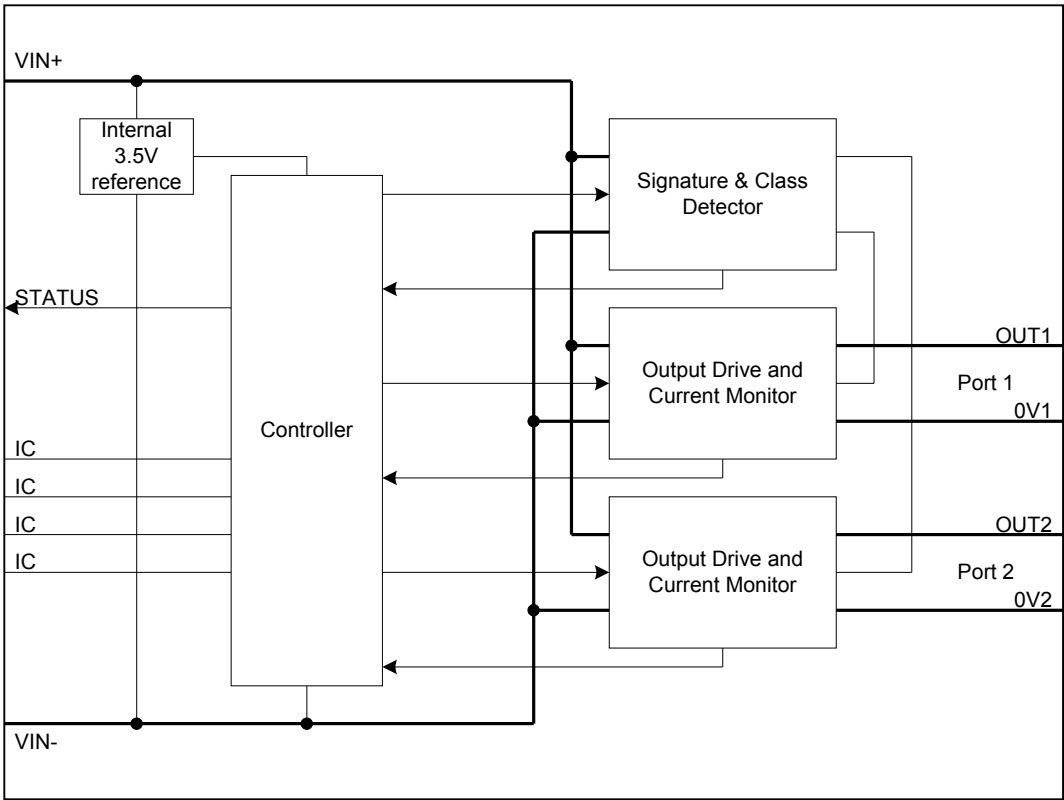
Figure 1: Block Diagram
