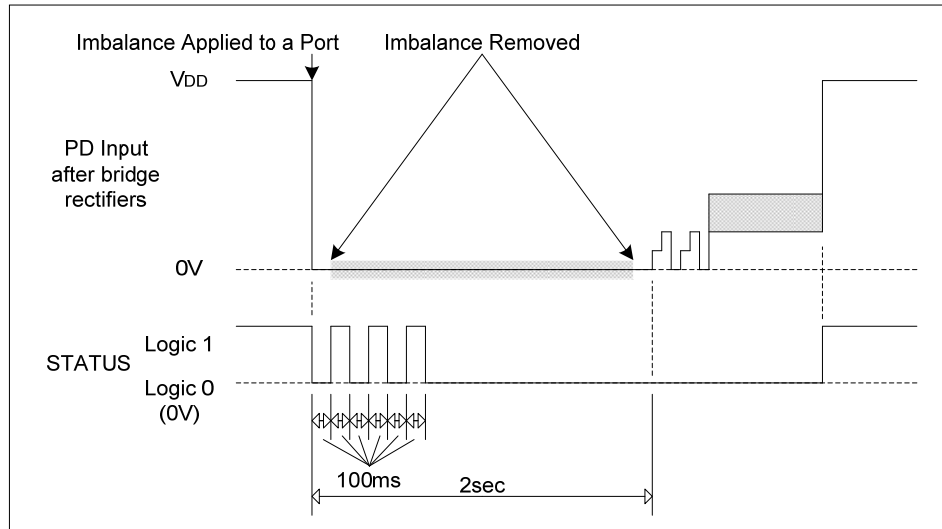
Figure 11: STATUS Output when an imbalance fault is detected
