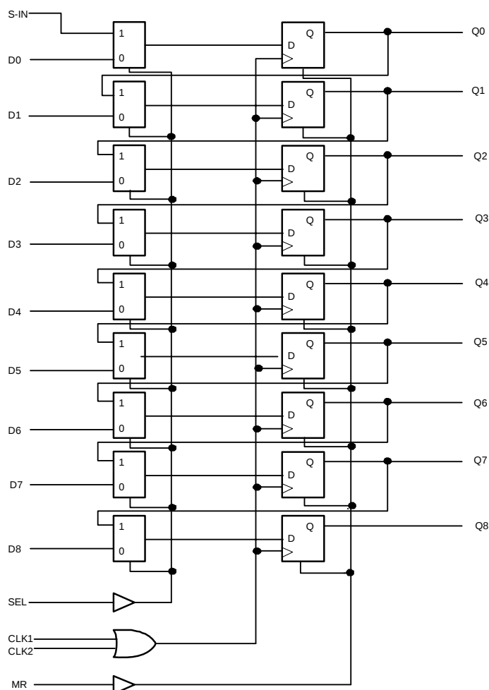
LOGIC SYMBOL
