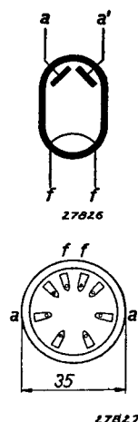
Fig. 2 Arrangement of electrodes and base connections.
