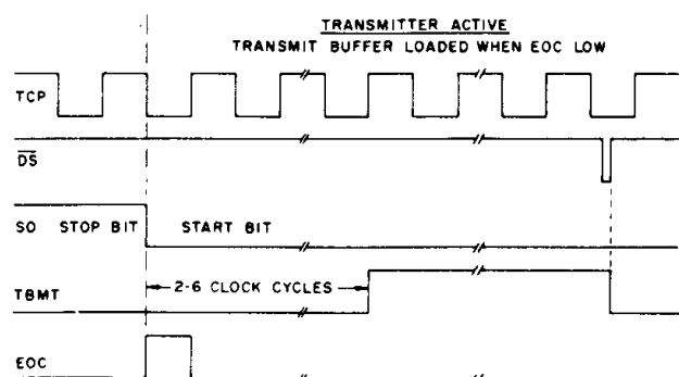
Fig.7 TRANSMITTER AT START BIT
