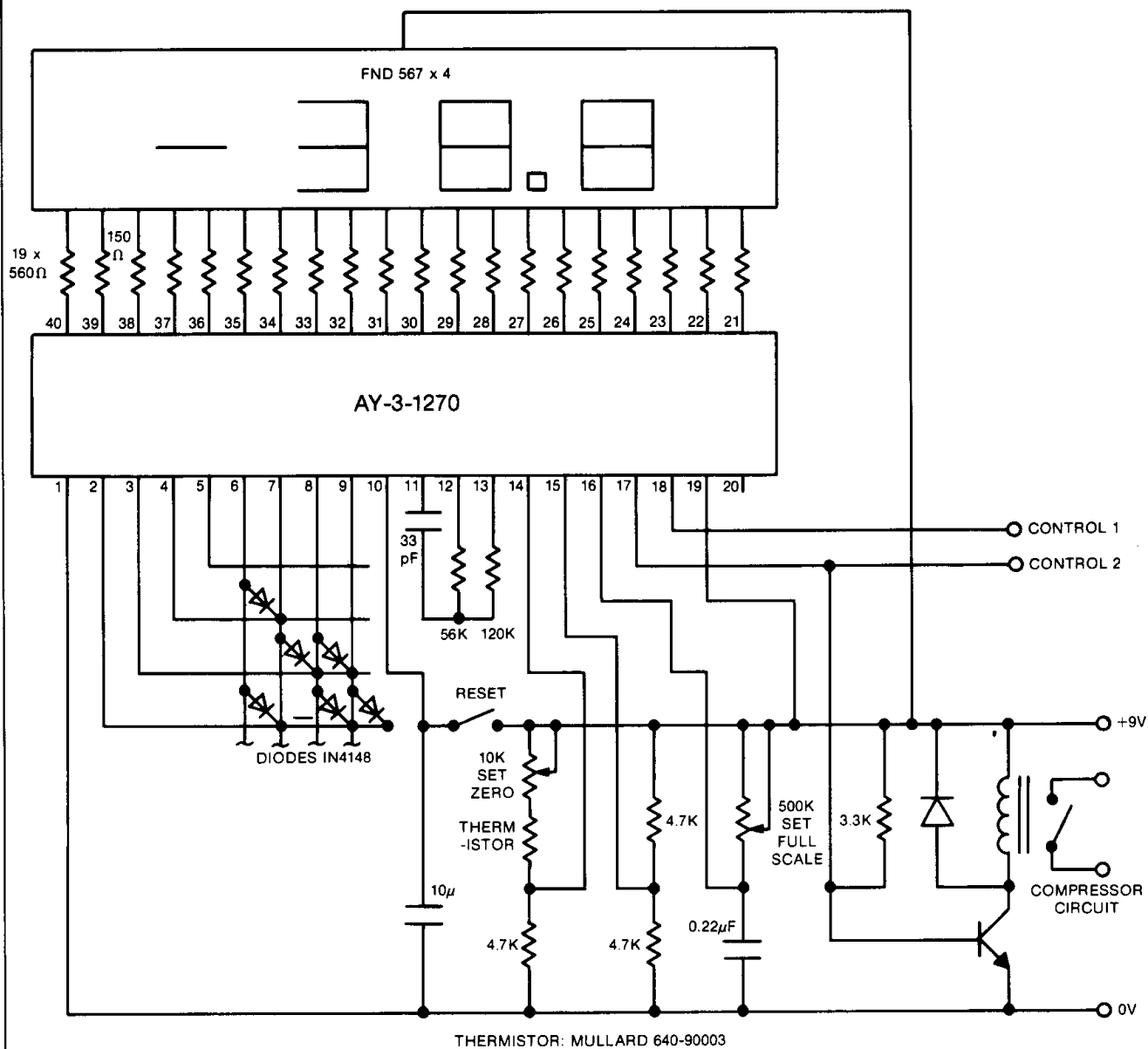
Fig. 9 THERMOMETER WITH LEAD DISPLAY
