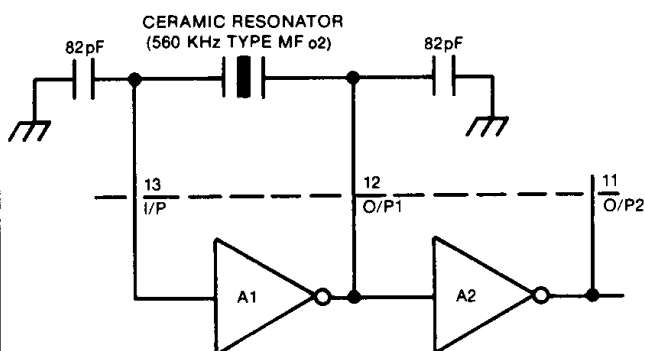
Fig. 1 TYPICAL OSCILLATOR CONFIGURATIONS
