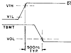
Fig.18 TBMT TURN-OFF
