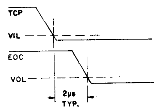
Fig.41 EOC TURN-OFF
