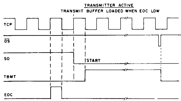
Fig.29 TRANSMITTER AT START BIT
