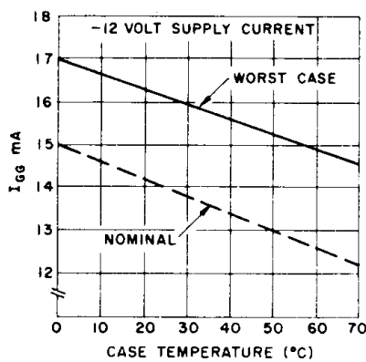
Fig.25 -12 VOLT SUPPLY CURRENT
