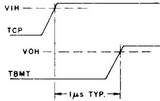
Fig.20 TBMT TURN-ON
