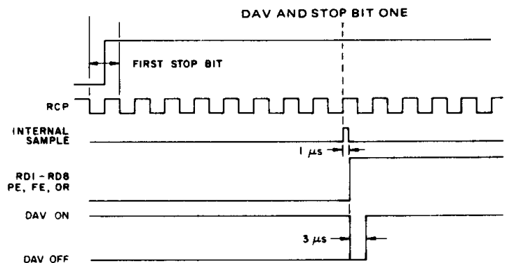
Fig.12 RECEIVER DURING 1st STOP BIT
