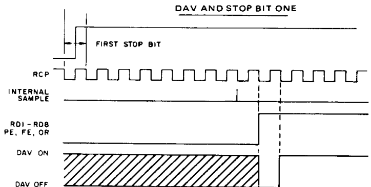
Fig.34 RECEIVER DURING 1ST STOP BIT
