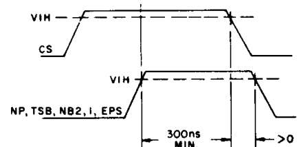
Fig.12 RECEIVER DURING 1st STOP BIT
