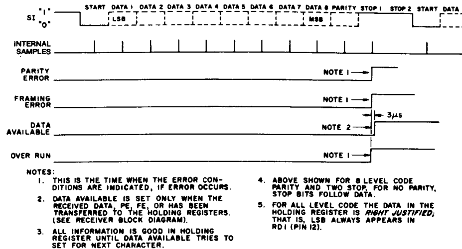
Fig.10 UAR/T RECEIVER TIMING
