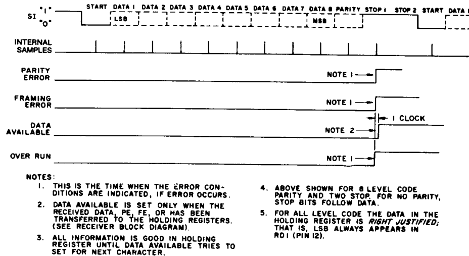
Fig.32 UAR/T — RECEIVER TIMING
