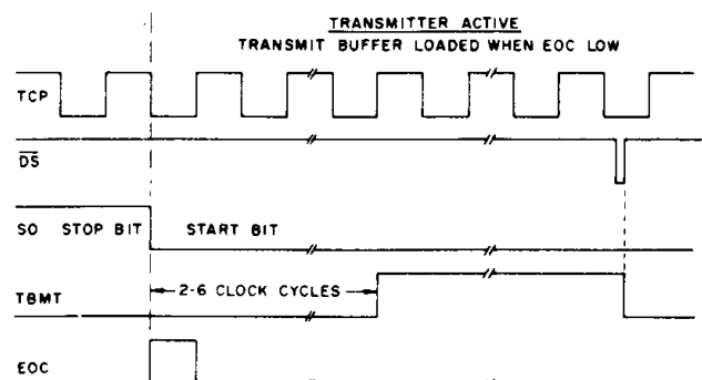
Fig.7 TRANSMITTER AT START BIT
