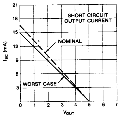
Fig.45 SHORT CIRCUIT OUTPUT CURRENT (only 1 output may be shorted at a time)
