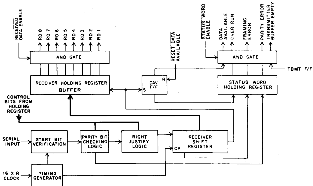
Fig.4 RECEIVER BLOCK DIAGRAM
