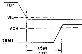
Fig.42 TBMT TURN-ON
