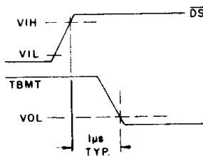
Fig.40 TBMT TURN-OFF
