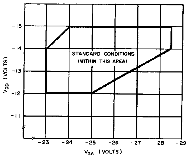
Fig. 2 OPERATING VOLTAGES
