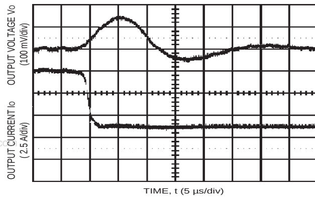
Figure 13. Typical Transient Response to Step Load Change at 2.5\text{ A}/\mu\text{s} from 100% to 50% of I_{O,\text{max}} at 3.3 V Input ( C_{\text{OUT}} = 1\text{ }\mu\text{F} ceramic, 10\text{ }\mu\text{F} Tantalum).
