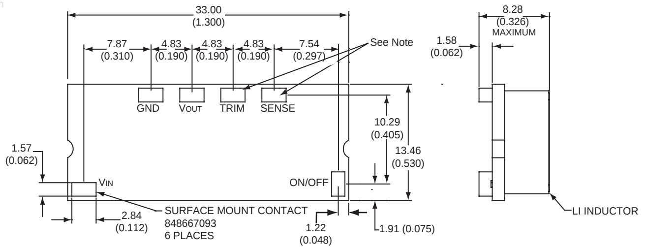
BOTTOM VIEW OF BOARD
