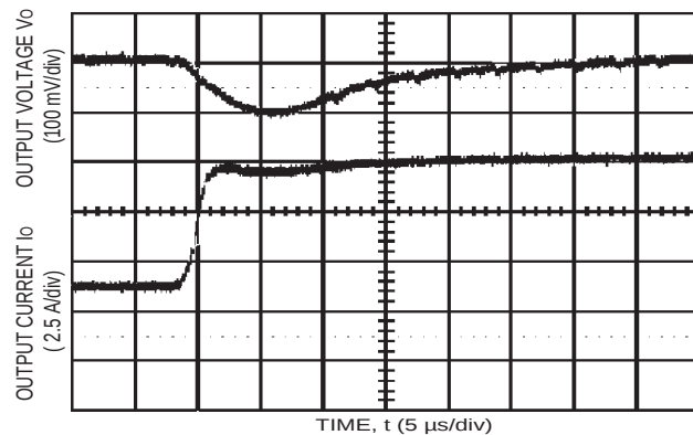
Figure 14. Typical Transient Response to Step Load Change at 2.5\text{ A}/\mu\text{s} from 50% to 100% of I_{O,\text{max}} at 3.3 V Input ( C_{\text{OUT}} = 1\text{ }\mu\text{F} ceramic, 10\text{ }\mu\text{F} Tantalum).
