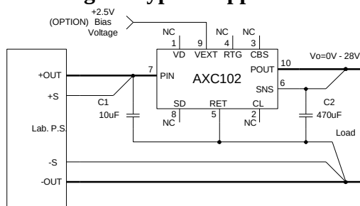
Fig.1 - Typical Application
