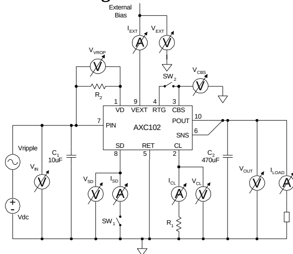
Fig.2 - Test Circuit
