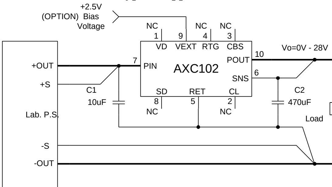
Fig.9B – Ultra Low Noise, High Efficiency Laboratory Switch-Mode Power Supply
