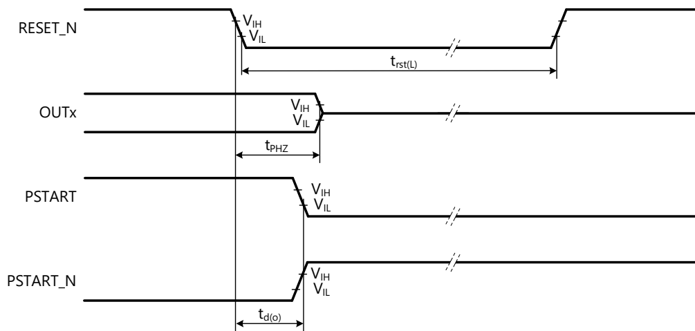
Figure 8. RESET_N Timing
