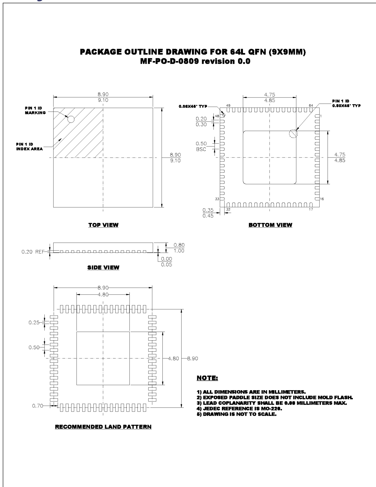
Figure 34. Package diagram AX5689GRK
