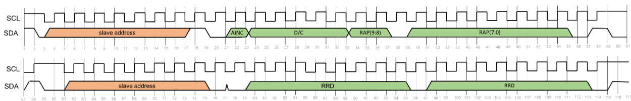
Figure 11. I2C read cycle
