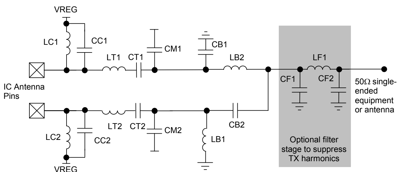
Figure 6 Structure of the antenna interface to 50 \Omega single-ended equipment or antenna
