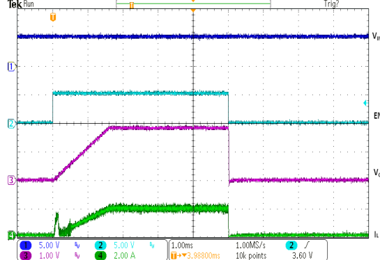
2A Load Start Up and Shutdown, 5V _{IN} to 1.8V _{OUT}
