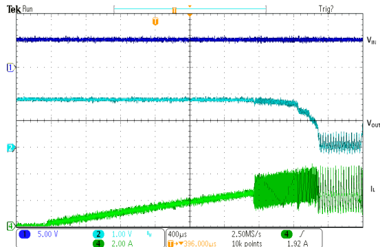
Output Short Circuit Test, 5V _{IN} to 1.8V _{OUT}
