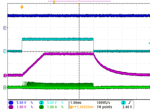
No Load Start Up and Shutdown, 5V _{IN} to 1.8V _{OUT}
