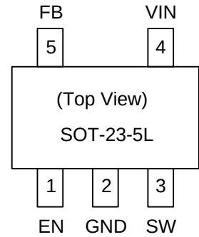
SOT-23-5L(A Type)
