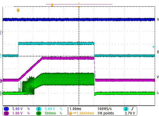
600mA Load Start Up and Shutdown, 5V _{IN} to 1.8V _{OUT}
