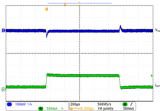
100mA~600mA Load Transient Test, 5V _{IN} to 1.8V _{OUT} , C3=330pF
