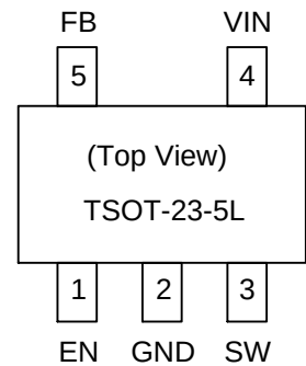
TSOT-23-5L(A Type)
