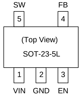
SOT-23-5L(B Type)
