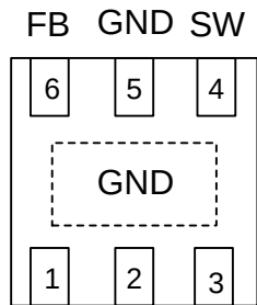
TDFN-6L (2*2)
