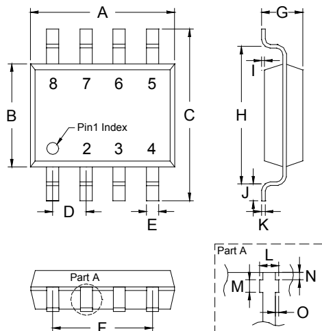
8-Lead SO-8 Plastic Surface Mounted Package AVANTICS Code: S
