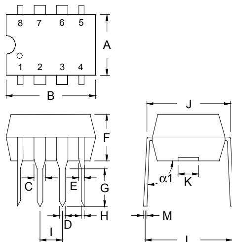
8-Lead DIP-8 Plastic Package AVANTICS Code: P
