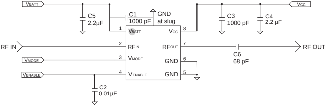
Figure 3: Application Circuit
