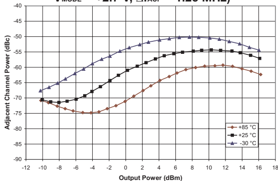
Figure 8: Adjacent Channel Power vs. P_{OUT} (f = 1780 MHz, V_{CC} = +4.2 V, V_{REF} = +3.0 V, V_{MODE} = +2.7 V, \Delta f_{ACP} = 1.25 MHz)
