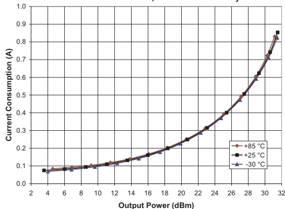
Figure 31: Current Consumption vs. P_{OUT} (f = 1765 \text{ MHz}, V_{CC} = +3.5 \text{ V}, V_{REF} = +2.85 \text{ V}, V_{MODE} = +2.7 \text{ V})
