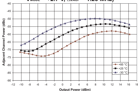
Figure 6: Adjacent Channel Power vs. P_{OUT} (f = 1780 MHz, V_{CC} = +3.5 V, V_{REF} = +3.0 V, V_{MODE} = +2.7 V, \Delta f_{ACP} = 1.25 MHz)
