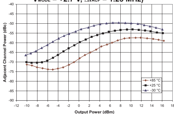
Figure 4: Adjacent Channel Power vs. P_{OUT} (f = 1780 MHz, V_{CC} = +3.0 V, V_{REF} = +3.0 V, V_{MODE} = +2.7 V, \Delta f_{ACP} = 1.25 MHz)
