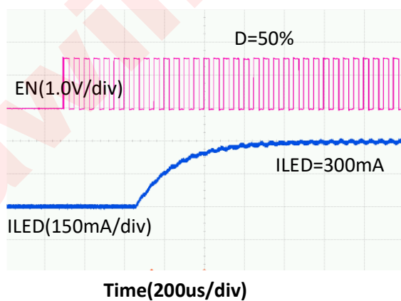
Figure 8. Startup Wave
