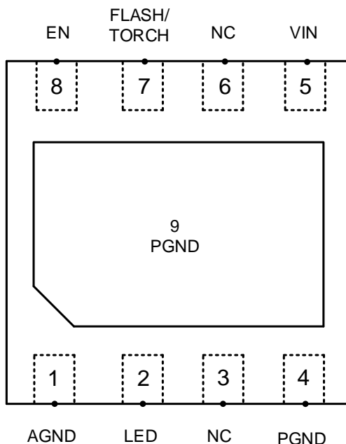
AW36406DNR Pin Configuration (Top View)
