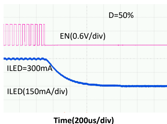
Figure 9. Shutdown Wave
