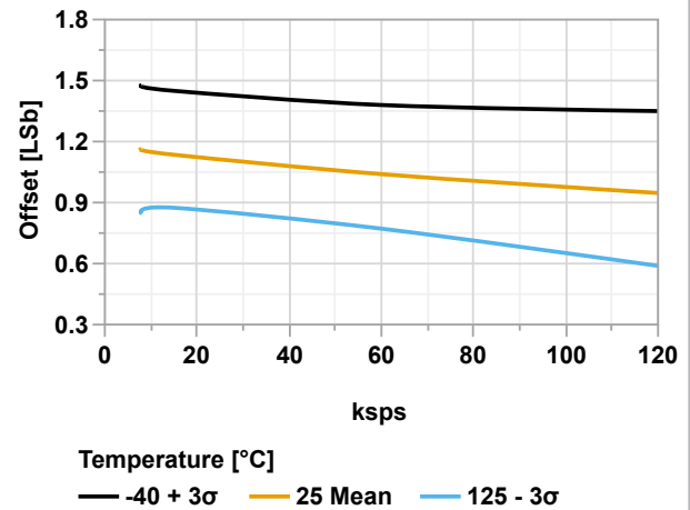
Figure 38-126. Offset Error vs. Sample Rate (ADC Differential Mode, V_{\text{REFA}} = V_{\text{DD}} = 3.6\text{V} )
