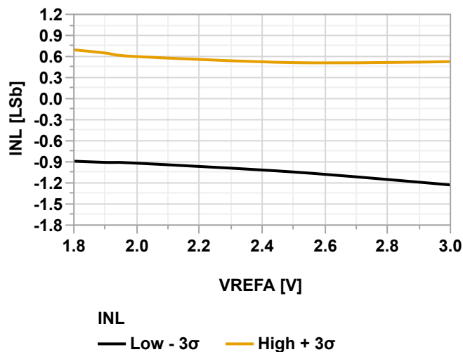
Figure 38-119. INL vs. V_{\text{REFA}} (ADC Single Ended Mode @60 kps, V_{\text{DD}} = 3.0\text{V} , T = 125^\circ\text{C} )
