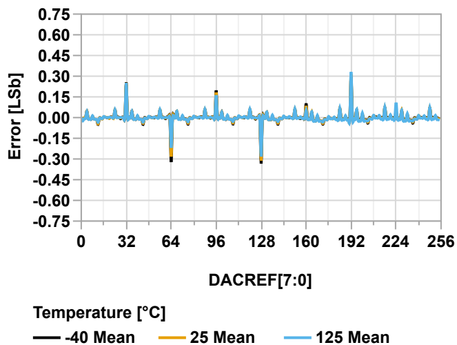
Figure 38-165. INL vs. DAC Code ( V_{\text{REFA}} = V_{\text{DD}} = 5.5\text{V} )
