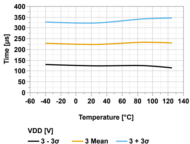
Figure 38-156. Settling Time vs. Temperature ( V_{\text{REFA}} = V_{\text{DD}} = 3.0\text{V} , Output Switch from 0\text{x}000 to 0\text{x}3\text{FF} )
