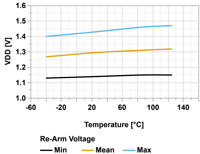
Figure 38-55. \overline{\text{POR}} Re-Arm Voltage vs. Temperature
