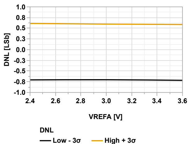
Figure 38-130. DNL vs. V_{\text{REFA}} (ADC Differential Mode @60 ksp/s, V_{\text{DD}} = 3.6\text{V} , T = 125^\circ\text{C} )
