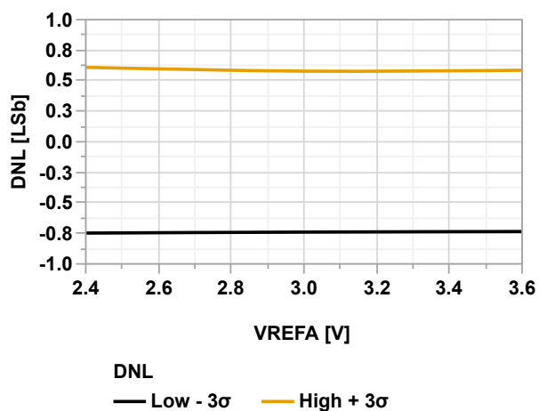
Figure 38-129. DNL vs. V_{\text{REFA}} (ADC Differential Mode @60 ksp/s, V_{\text{DD}} = 3.6\text{V} , T = 85^\circ\text{C} )
