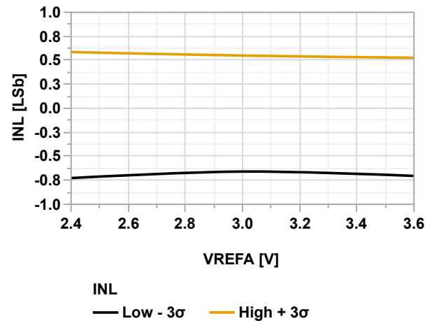
Figure 38-134. INL vs. V_{\text{REFA}} (ADC Differential Mode @60 ksp/s, V_{\text{DD}} = 3.6\text{V} , T = 125^\circ\text{C} )
