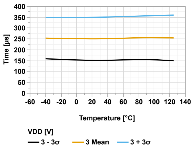
Figure 38-157. Settling Time vs. Temperature ( V_{\text{REFA}} = V_{\text{DD}} = 3.0\text{V} , Output Switch from 0\text{x}3\text{FF} to 0\text{x}000 )
