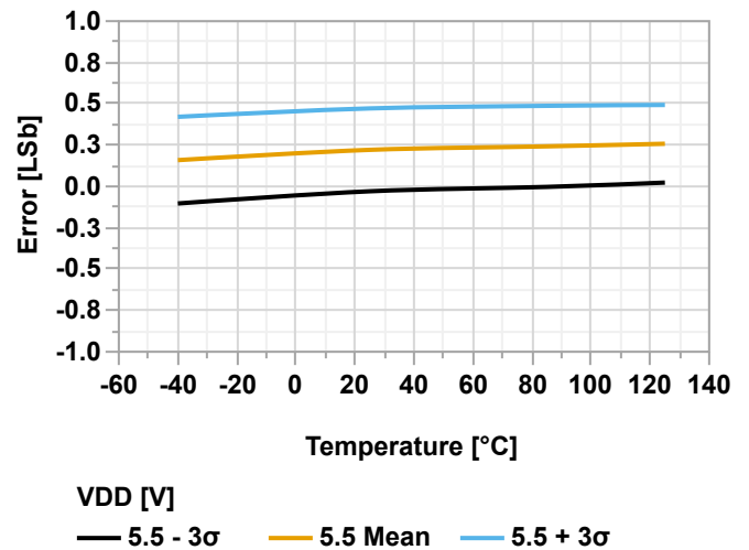
Figure 38-161. Offset Error vs. Temperature ( V_{\text{REFA}} = V_{\text{DD}} = 5.5\text{V} )
