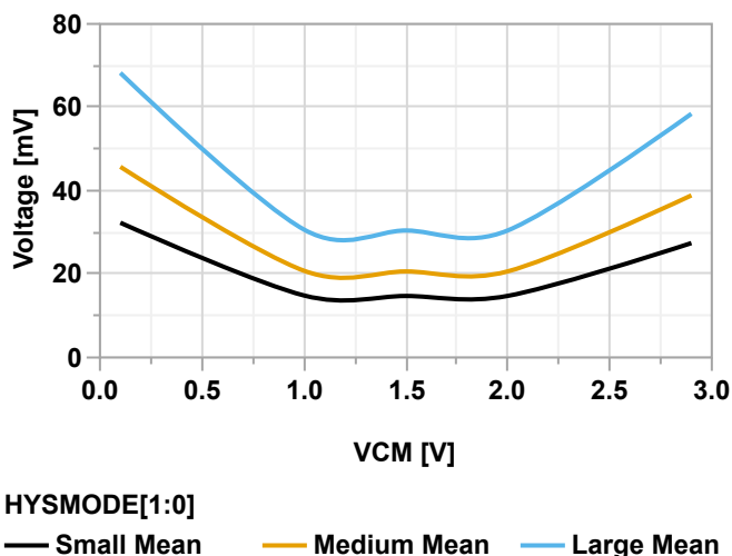
Figure 38-145. Input Hysteresis vs. Common Mode Voltage ( V_{DD} = 3.0V )
