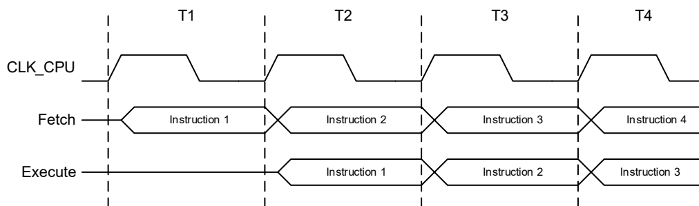
Figure 6-2. The Parallel Instruction Fetches and Executions
