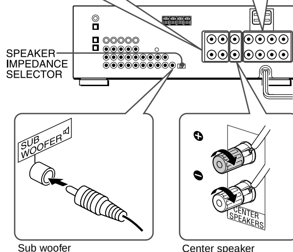
Sub woofer
