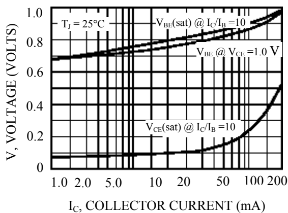
Figure 3. "ON" Voltages
