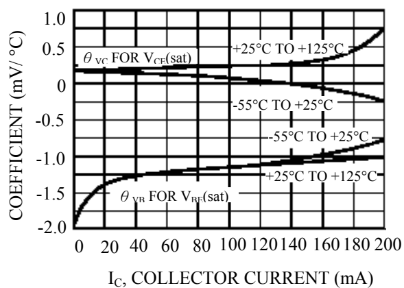
Figure 4. Temperature Coefficients
