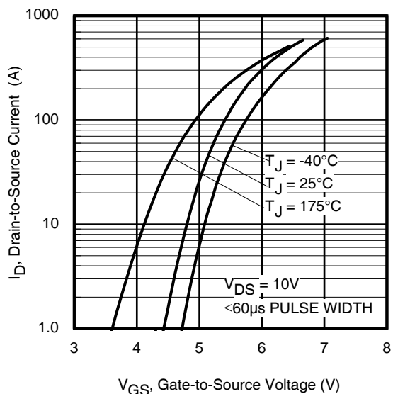
Fig 5. Transfer Characteristics
