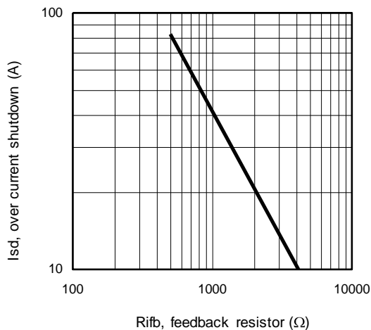
Figure 11 – Ids (A) Vs Rfcb (Ω)
