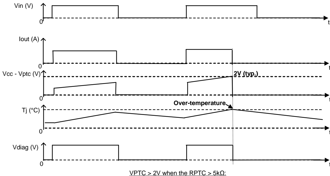
Figure 2: Protection PTC
