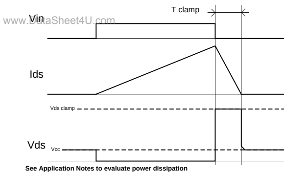
Figure 3 – Active clamp waveforms
