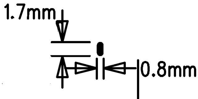
Fig.2 Pad dimension
