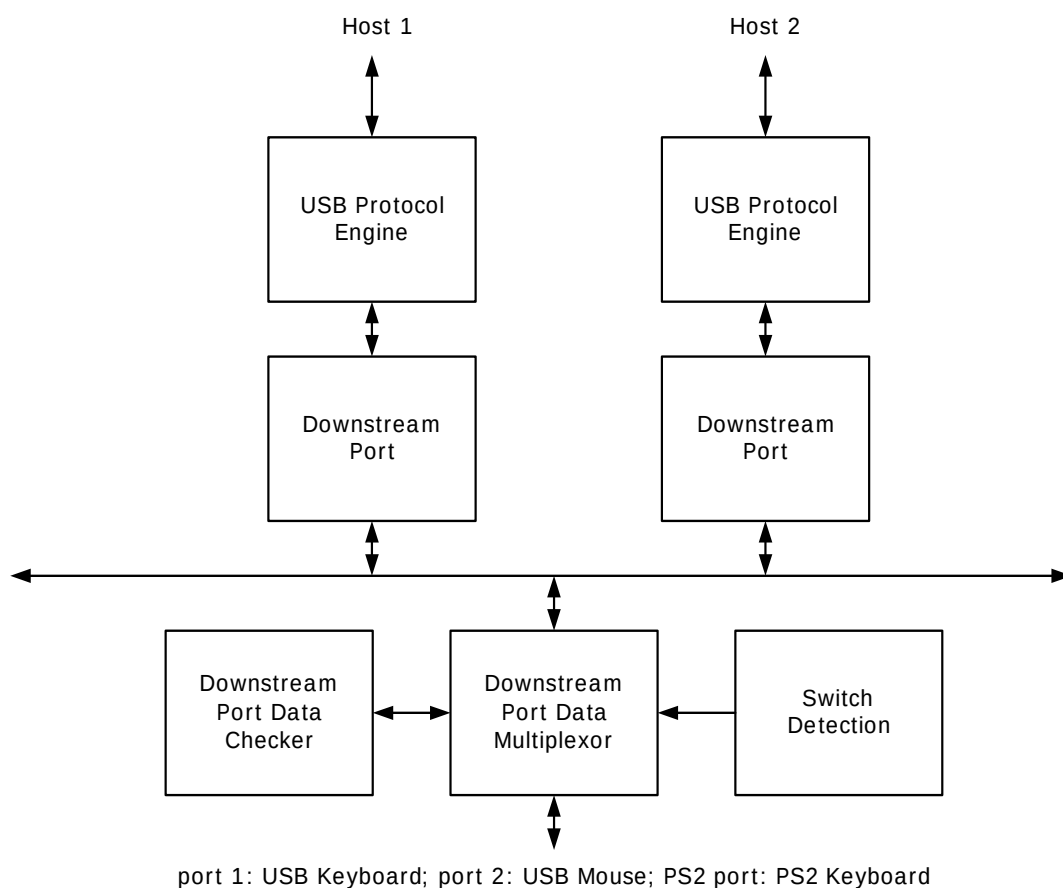
Figure 4.1 AU9226 Block Diagram
