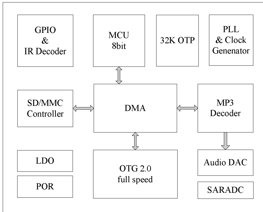
Figure 1 AU6860M Functional Block Diagram
