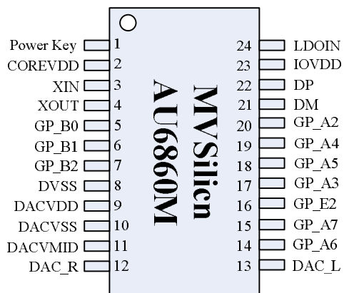
Figure 3 Package Diagram (TSSOP24 / TOP View)
