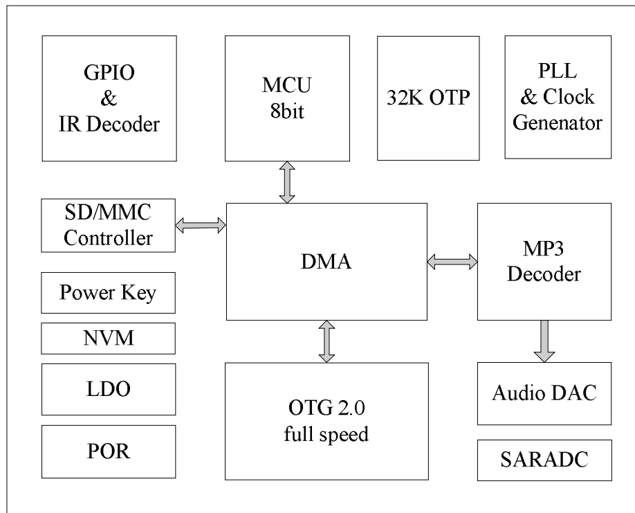
Figure 1 AU6860L Functional Block Diagram
