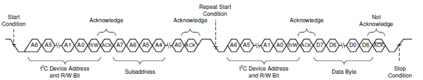
Figure 15. Random Read Transfer
