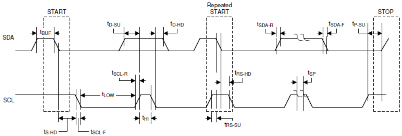
Figure 3. I²C Communication Port Timing Diagram
