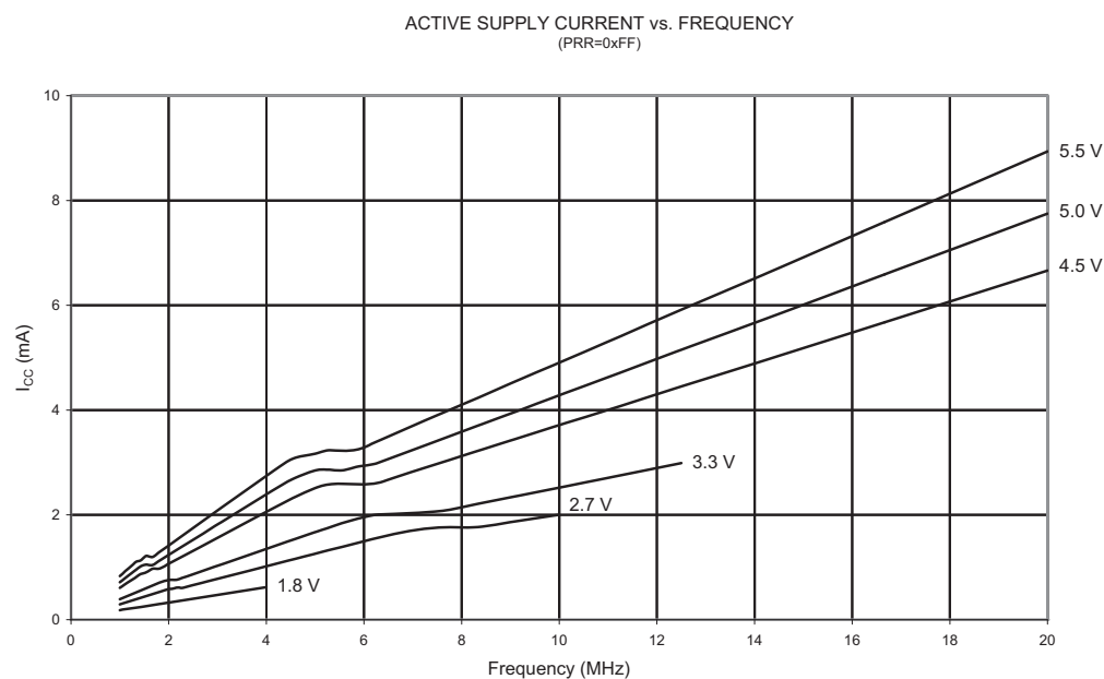
Figure 21-4. Active Supply Current vs. Frequency (1 - 20 MHz)
