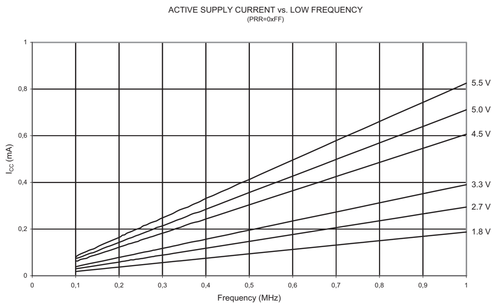
Figure 21-3. Active Supply Current vs. Low Frequency (0.1 - 1.0 MHz)
