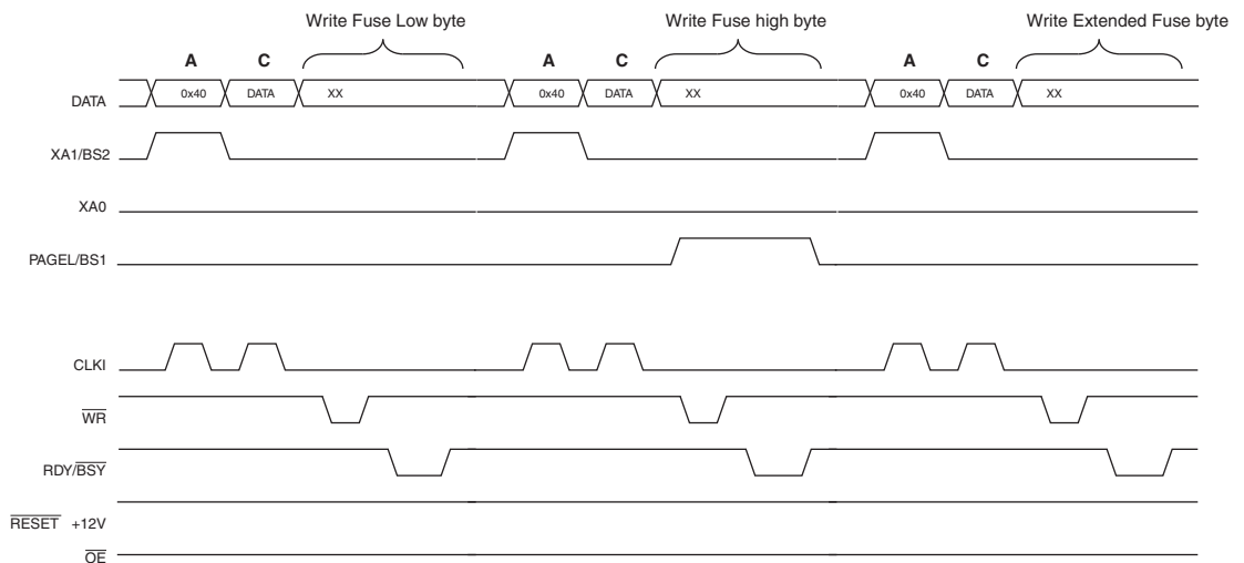
Figure 19-5. Programming the FUSES Waveforms
