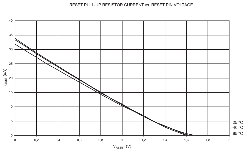
Figure 21-22. Reset Pull-up Resistor Current vs. Reset Pin Voltage ( V_{CC} = 1.8V )
