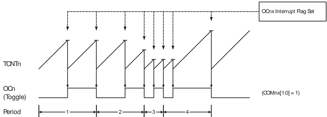
Figure 12-5. CTC Mode, Timing Diagram
