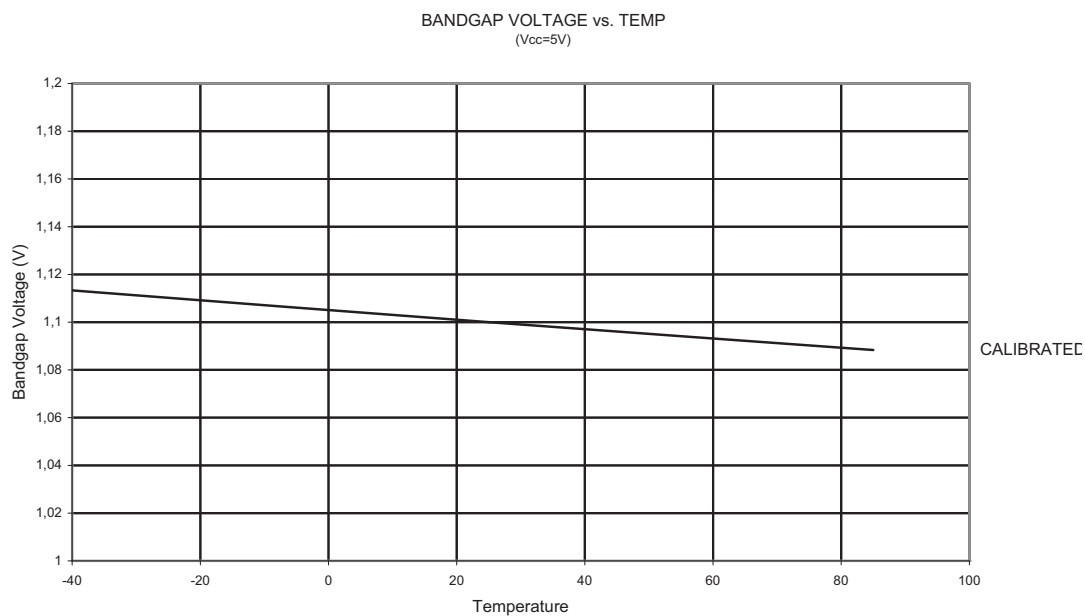
Figure 21-43. Bandgap Voltage vs. Temperature
