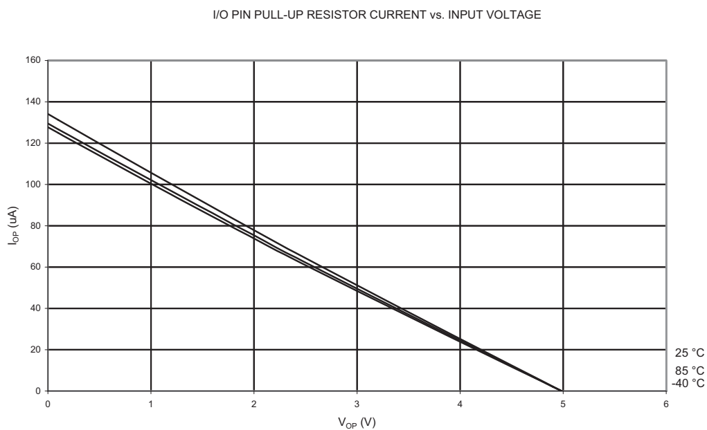
Figure 21-21. Pull-up Resistor Current vs. Input Voltage (I/O Pin, V_{CC} = 5V )
