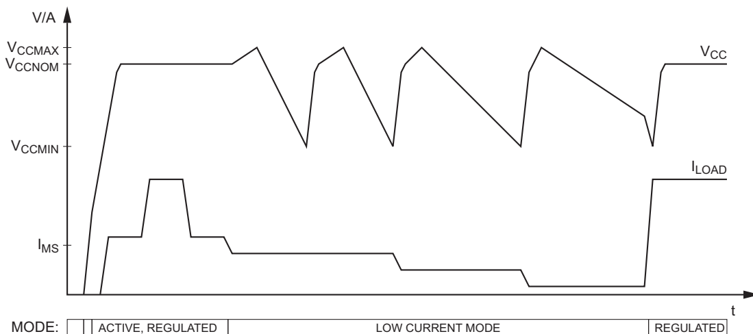
Figure 8-5. Output Voltage vs. Load Current of Boost Converter.
