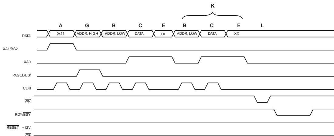
Figure 19-4. Programming the EEPROM Waveforms
