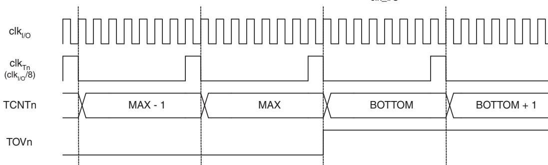
Figure 12-9. Timer/Counter Timing Diagram, with Prescaler ( f_{\text{clk}_{I/O}}/8 )
