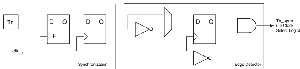
Figure 13-1. T_n Pin Sampling
