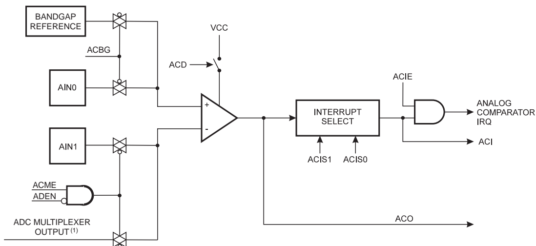
Figure 15-1. Analog Comparator Block Diagram
