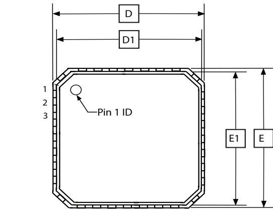
TOP VIEW W
