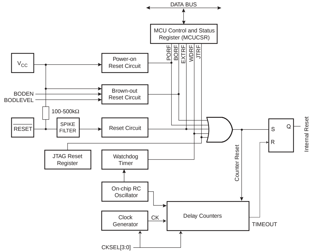
Figure 24. Reset Logic
