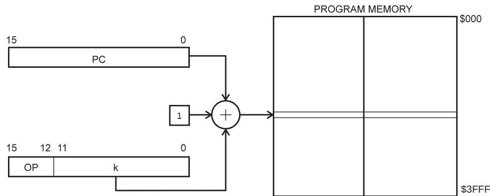
Relative Program Addressing, RJMP and RCALL Figure 20. Relative Program Memory Addressing
