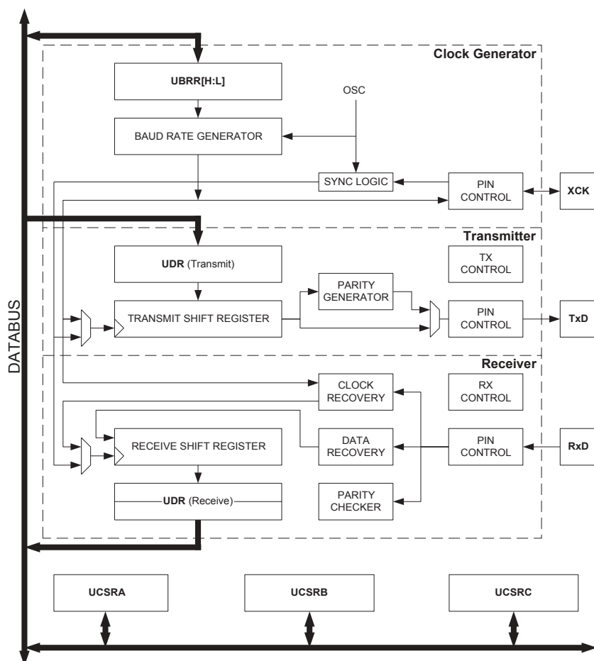
Figure 45. USART Block Diagram
