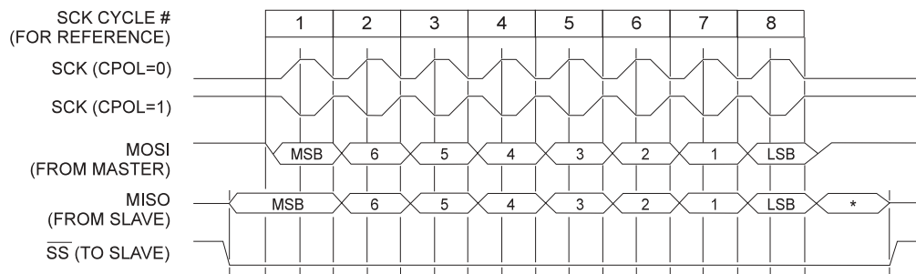
Figure 43. SPI Transfer Format with CPHA = 0 and DORD = 0 (1)
