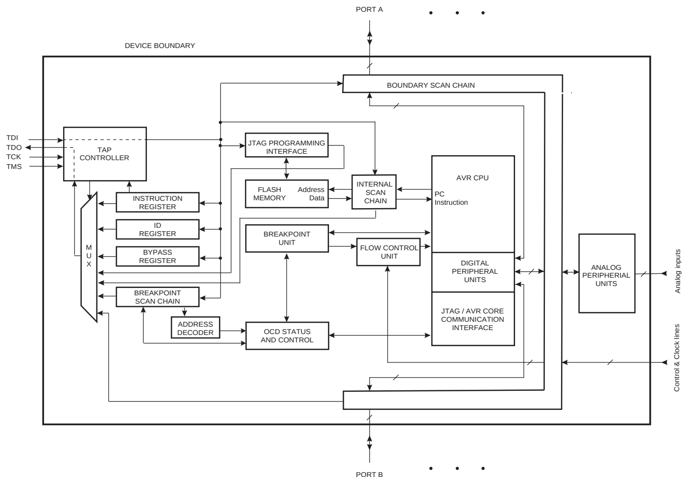
Figure 85. Block Diagram
