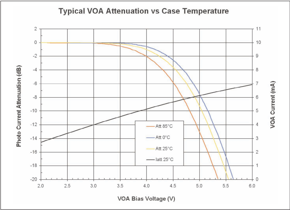
Figure [5] Typical VOA attenuation.
