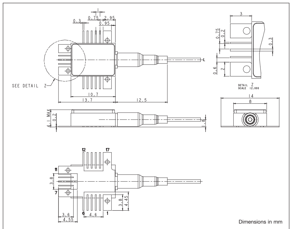
Figure [2] Outline diagram (Illustration only. For full details, refer to appropriate assembly drawing).
