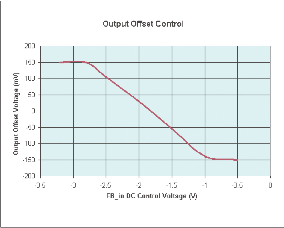
Figure [6] FB_in transfer function.
