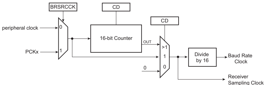
Figure 44-3. Baud Rate Generator
