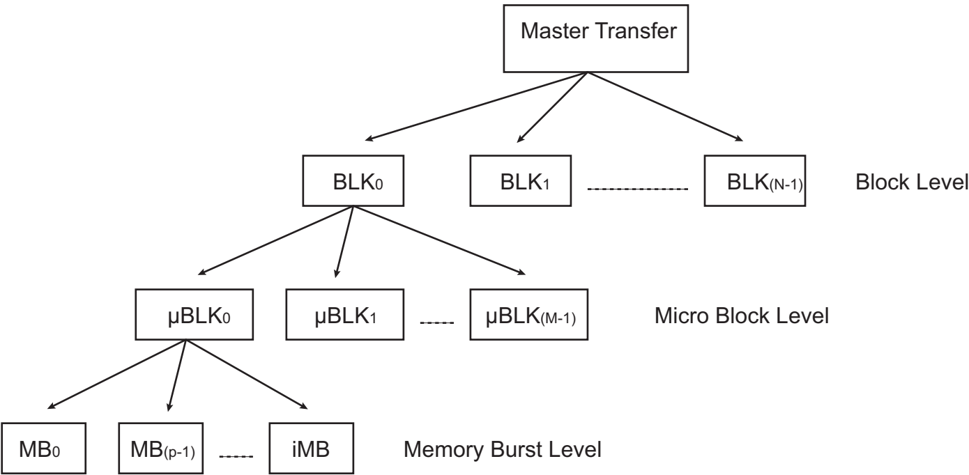
Figure 34-2. XDMAC Memory Transfer Hierarchy
