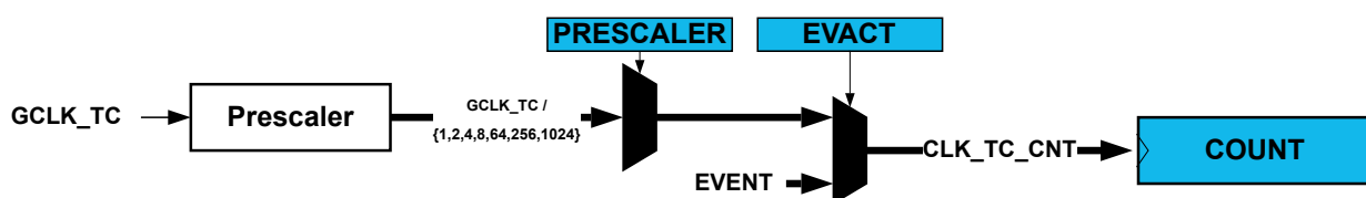
Figure 35-2. Prescaler
