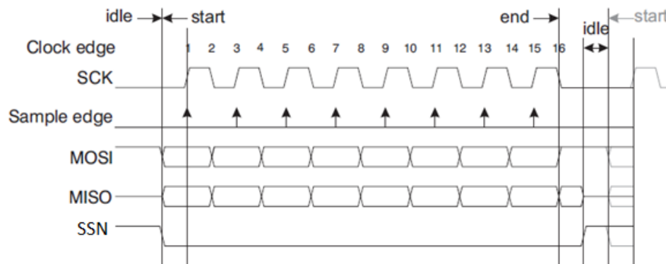
Figure 18-3. SCK_POLARITY = 0; SCK_PHASE = 0
