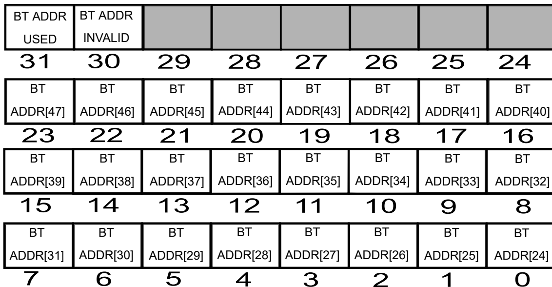
Figure 7-1. Bank 5 Block 0
