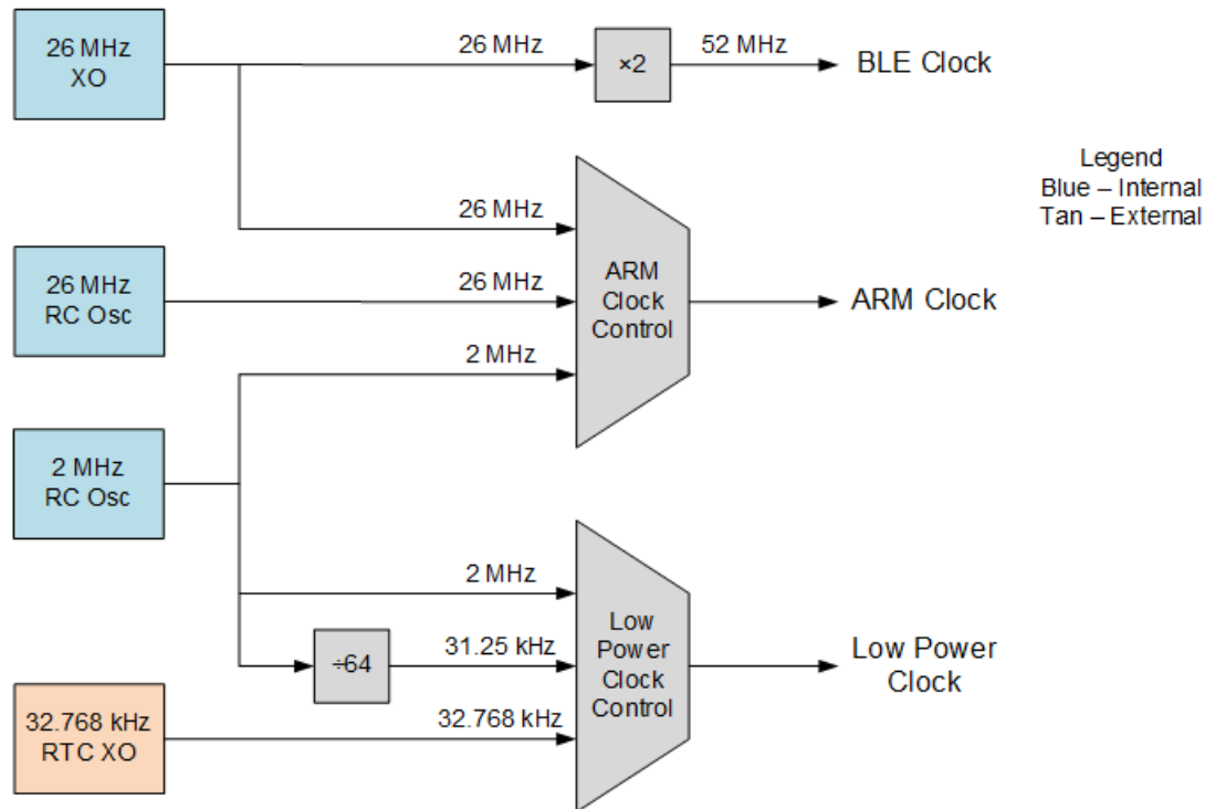
Figure 9-1. Clock Architecture
