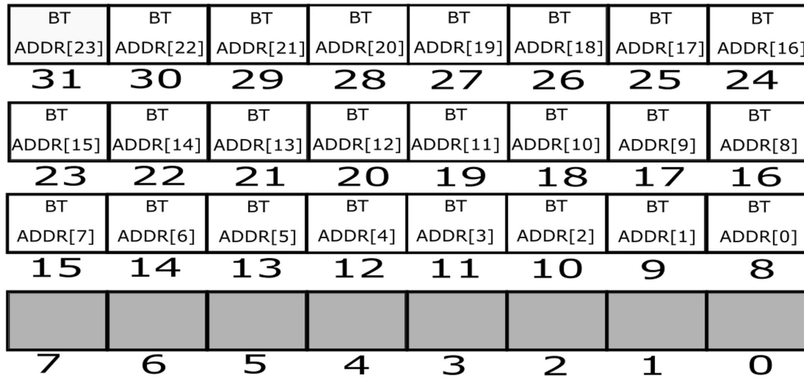
Figure 7-2. Bank 5 Block 1
