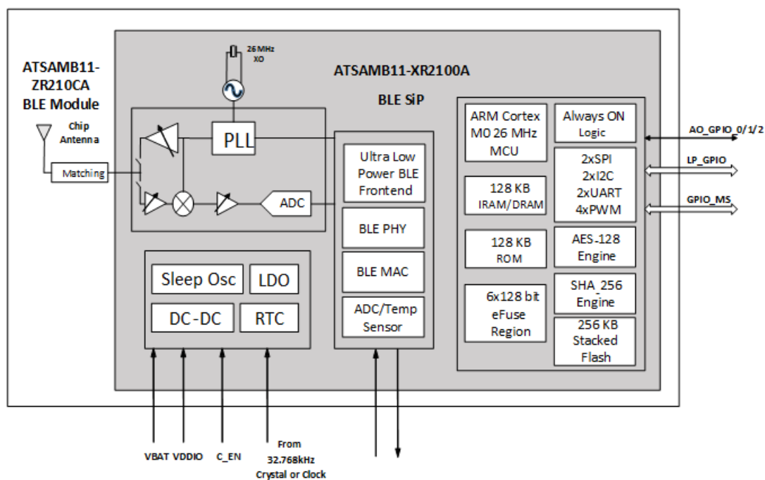
Figure 3-1. Block Diagram
