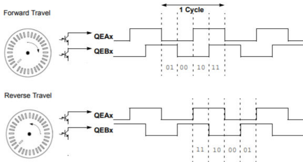
Figure 21-1. Quadrature Decoder Interface Signals
