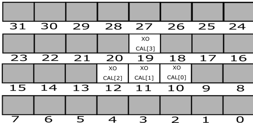
Figure 7-3. Bank 5 Block 3
