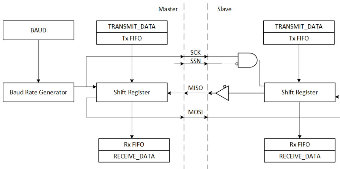
Figure 18-1. Full-Duplex SPI Master Slave Interconnection
