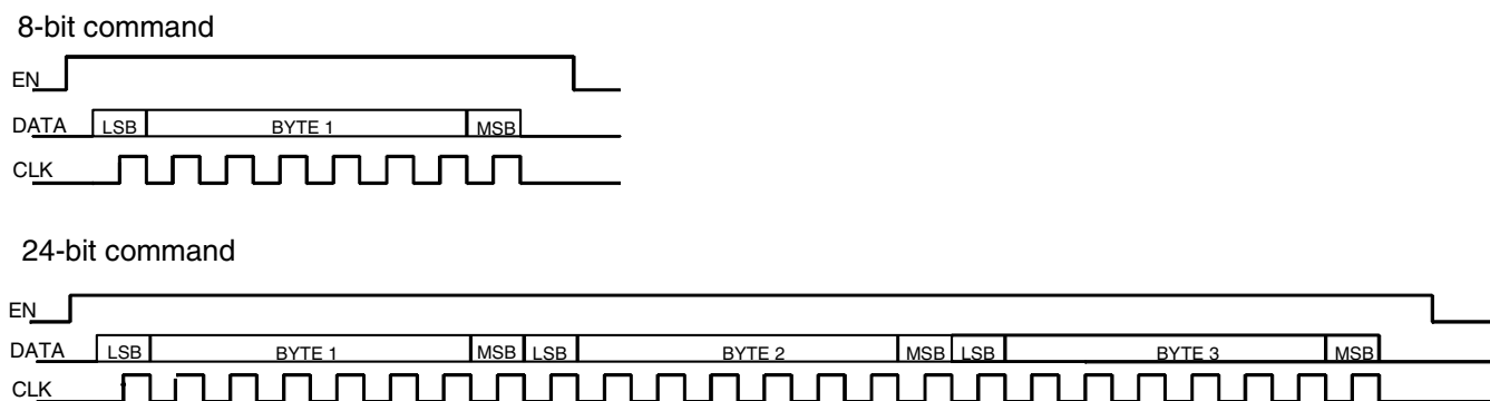
Figure 10. Pulse Diagram
