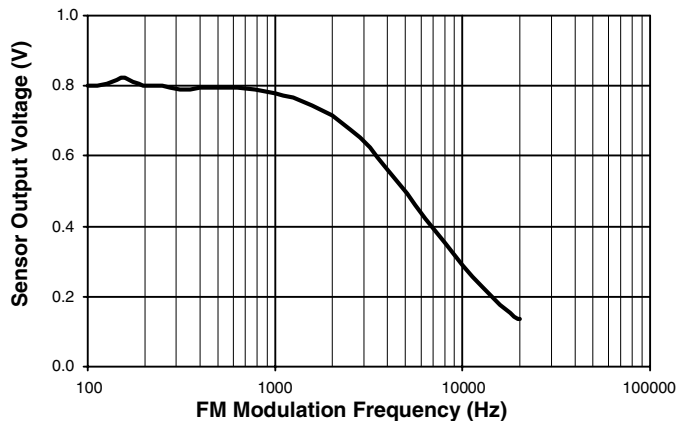
Figure 16. Deviation Sensor Frequency Response
