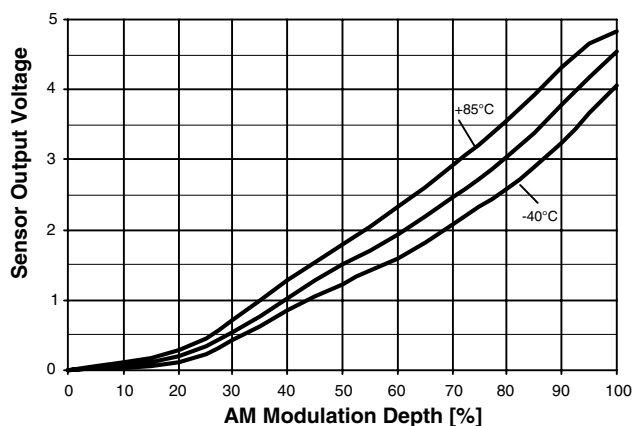
Figure 13. Multipath Sensor
