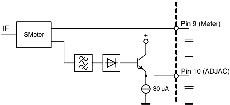
Figure 8. Adjacent Channel Sensor
