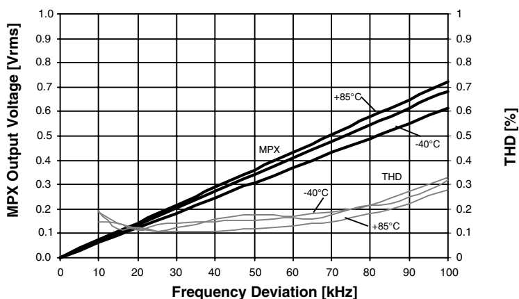
Figure 12. FM Demodulator
