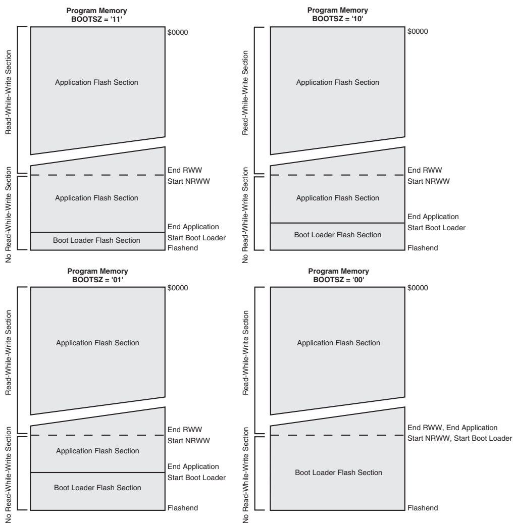
Figure 113. Memory sections (1)
