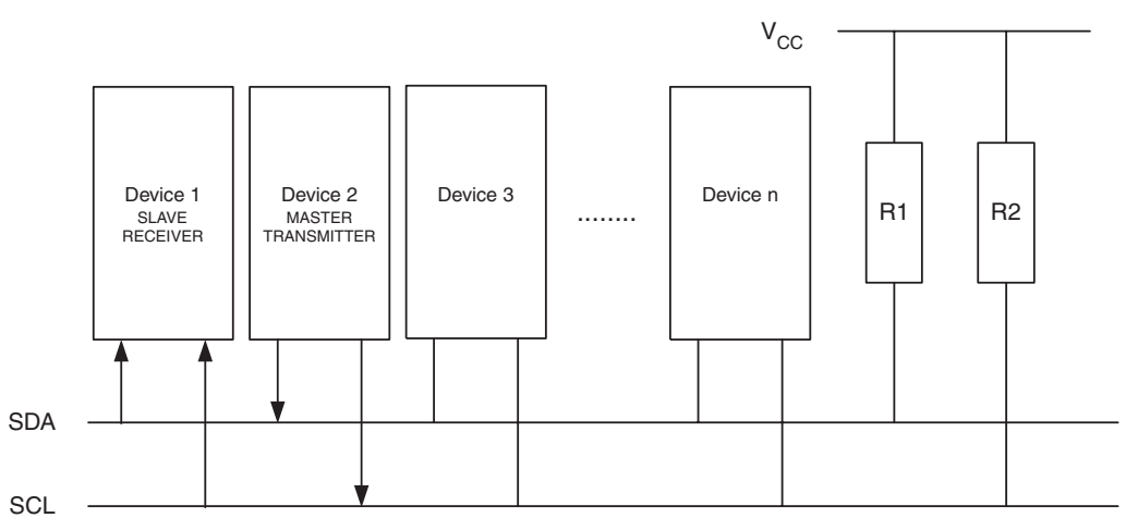
Figure 90. Data Transfer in Slave Receiver Mode
