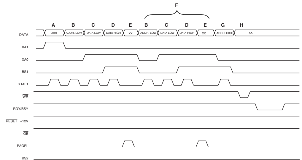
Figure 117. Programming the Flash Waveforms (1)
