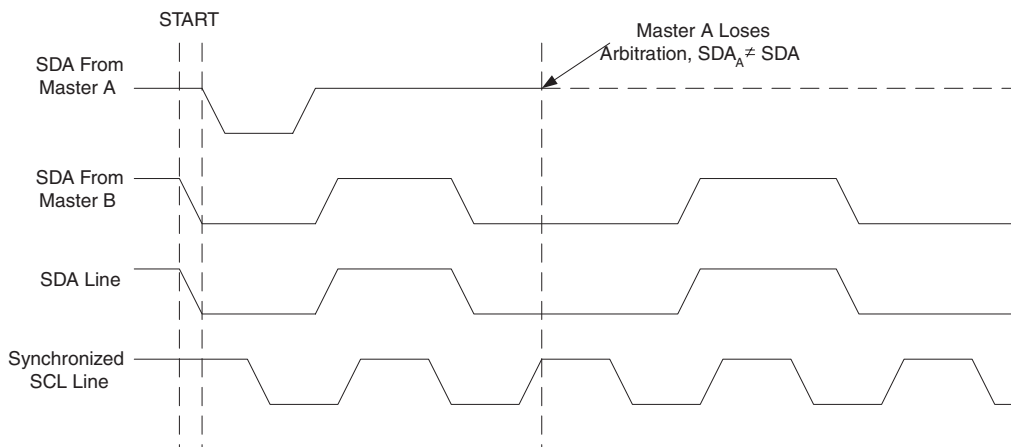
Figure 83. Arbitration Between Two Masters
