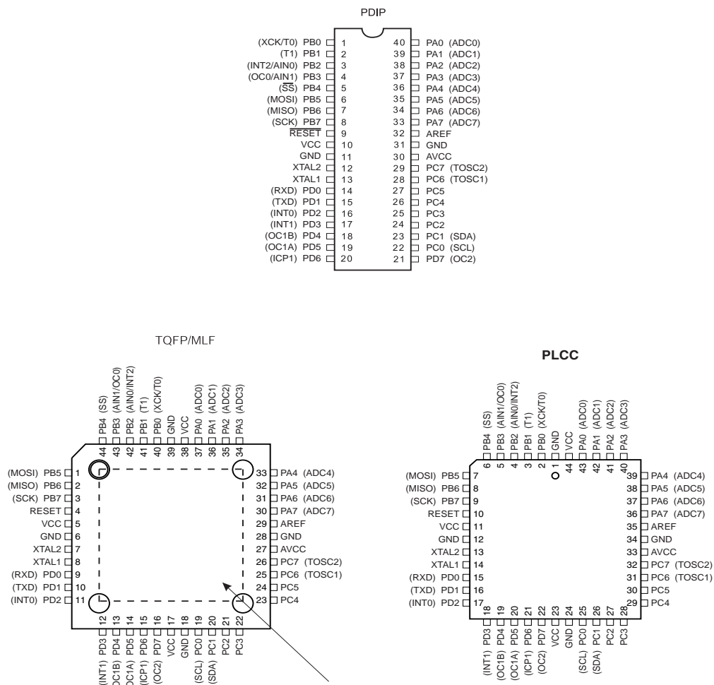
Figure 1. Pinout ATmega8535
