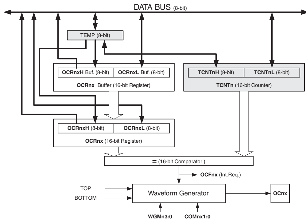
Figure 43. Output Compare Unit, Block Diagram
