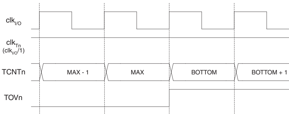
Figure 34. Timer/Counter Timing Diagram, no Prescaling
