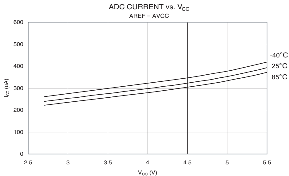
Figure 188. ADC Current vs. V_{CC} (AREF = AVCC)
