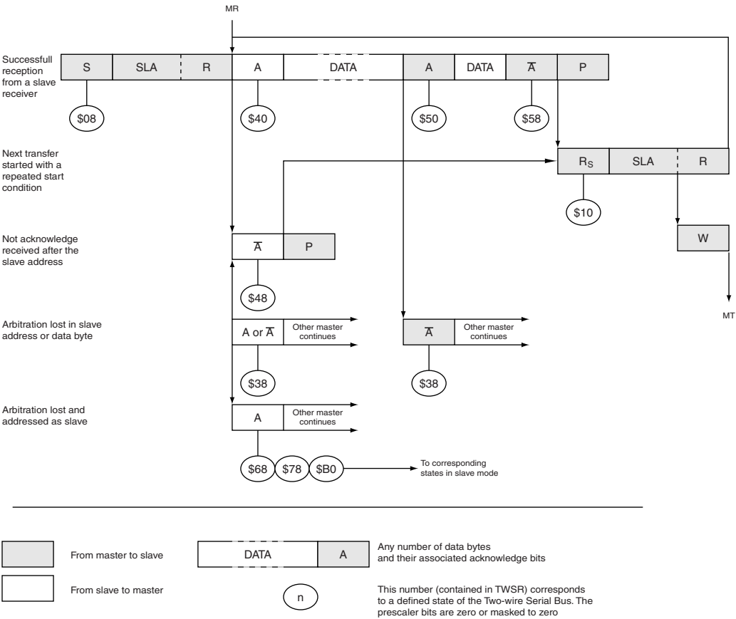
Figure 89. Formats and States in the Master Receiver Mode
