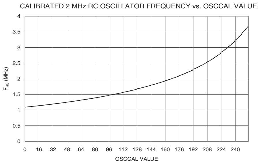
Figure 183. Calibrated 2 MHz RC Oscillator Frequency vs. Oscal Value
