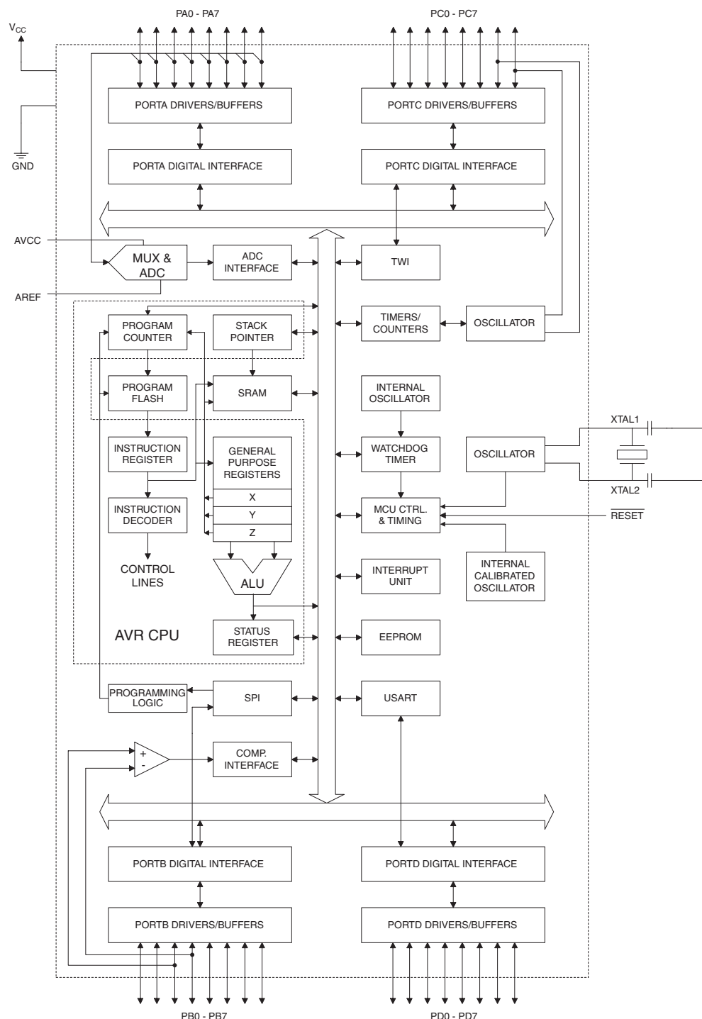
Figure 2. Block Diagram
