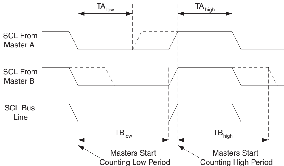
Figure 82. SCL Synchronization Between Multiple Masters
