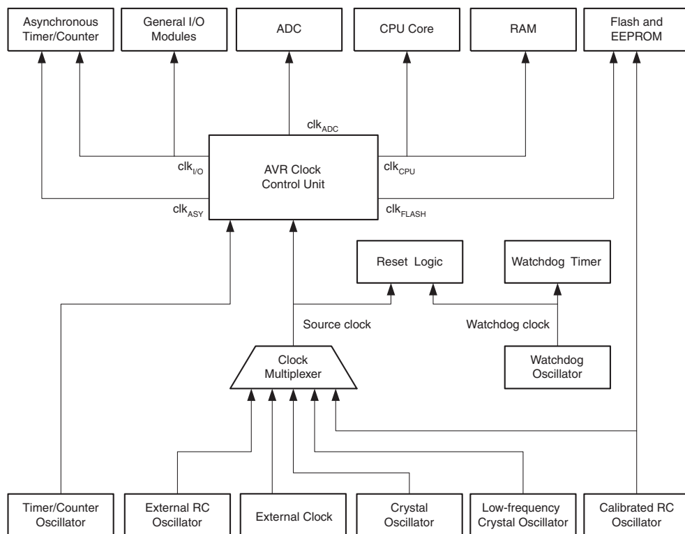
Figure 11. Clock Distribution
