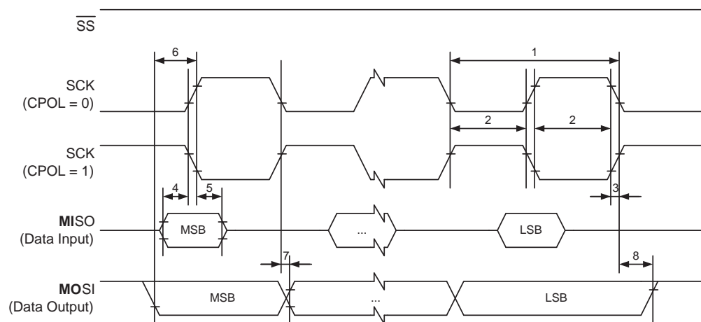
Figure 28-5. SPI Interface Timing Requirements (Master Mode)
