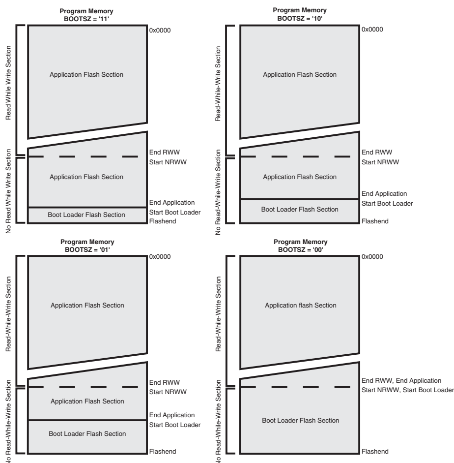
Figure 94. Memory Sections (1)
